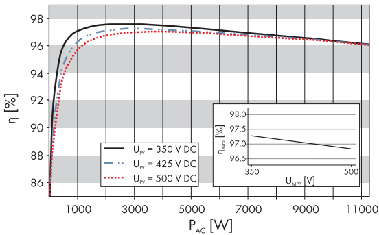
Efficiency curve
